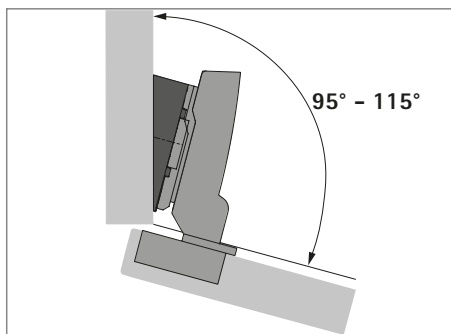
Applications with cabinet body angle of 95° - 115°
