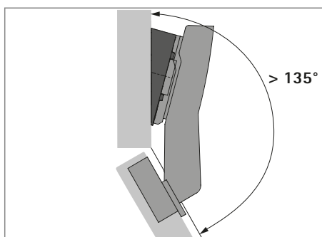
Applications with cabinet body angle of greater than 135°
