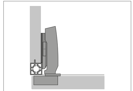
Applications with Cadro frame system
