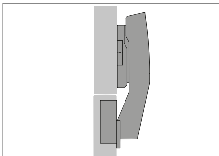
Applications for corner cabinets
