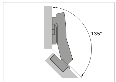
Applications with cabinet body angle of 135°
