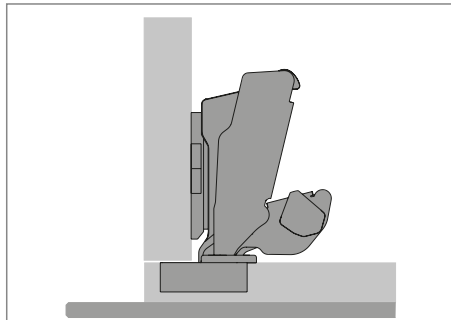
Applications with protruding front
