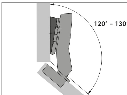
Applications with cabinet body angle of 120° - 130°
