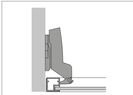
Applications for aluminium framed doors
